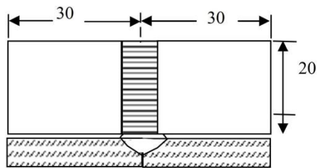
Fig.5: Welding specimen for practice
