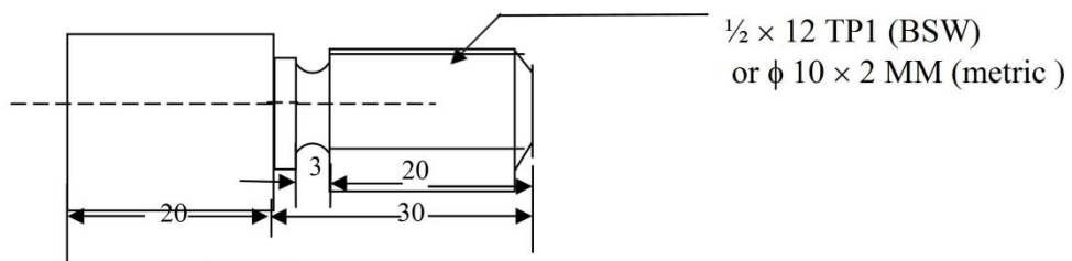
Fig.2: Job for practice on a lathe
