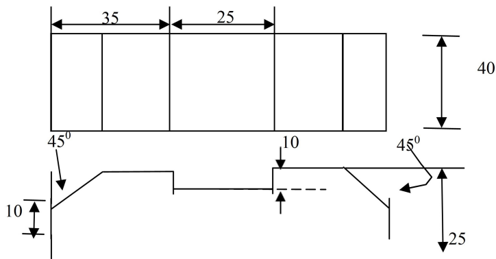
Fig.4: Job for making a pattern
