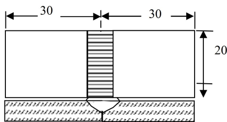
Fig.5: Welding specimen for practice
