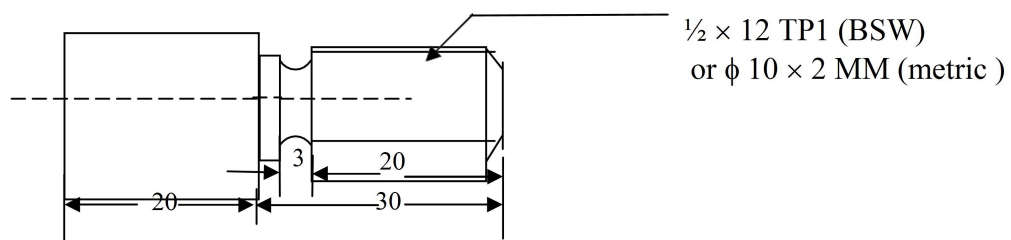
Fig.2: Job for practice on a lathe
